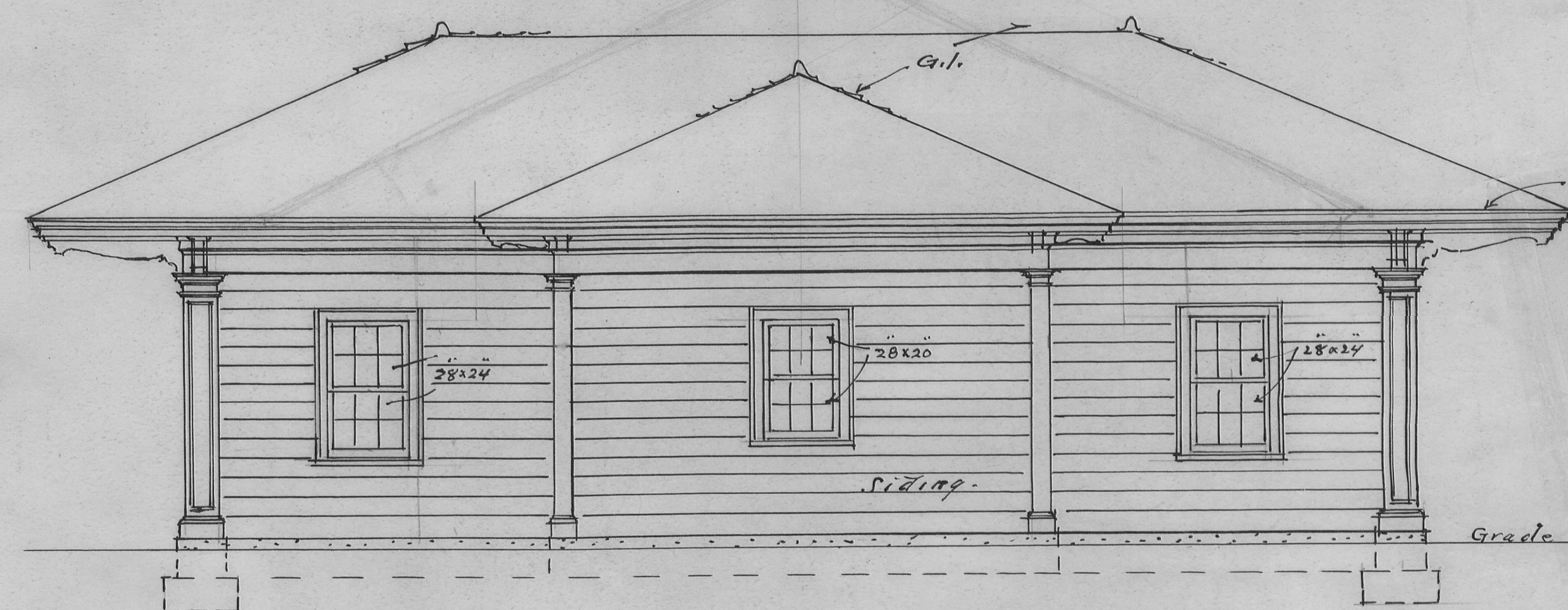
SOUTH ELEVATION.
