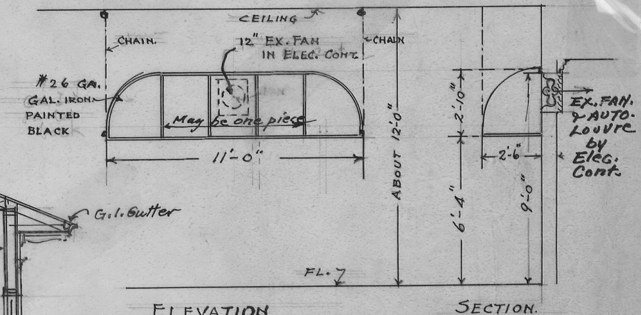
HOOD SECTION 1/2" scale.
