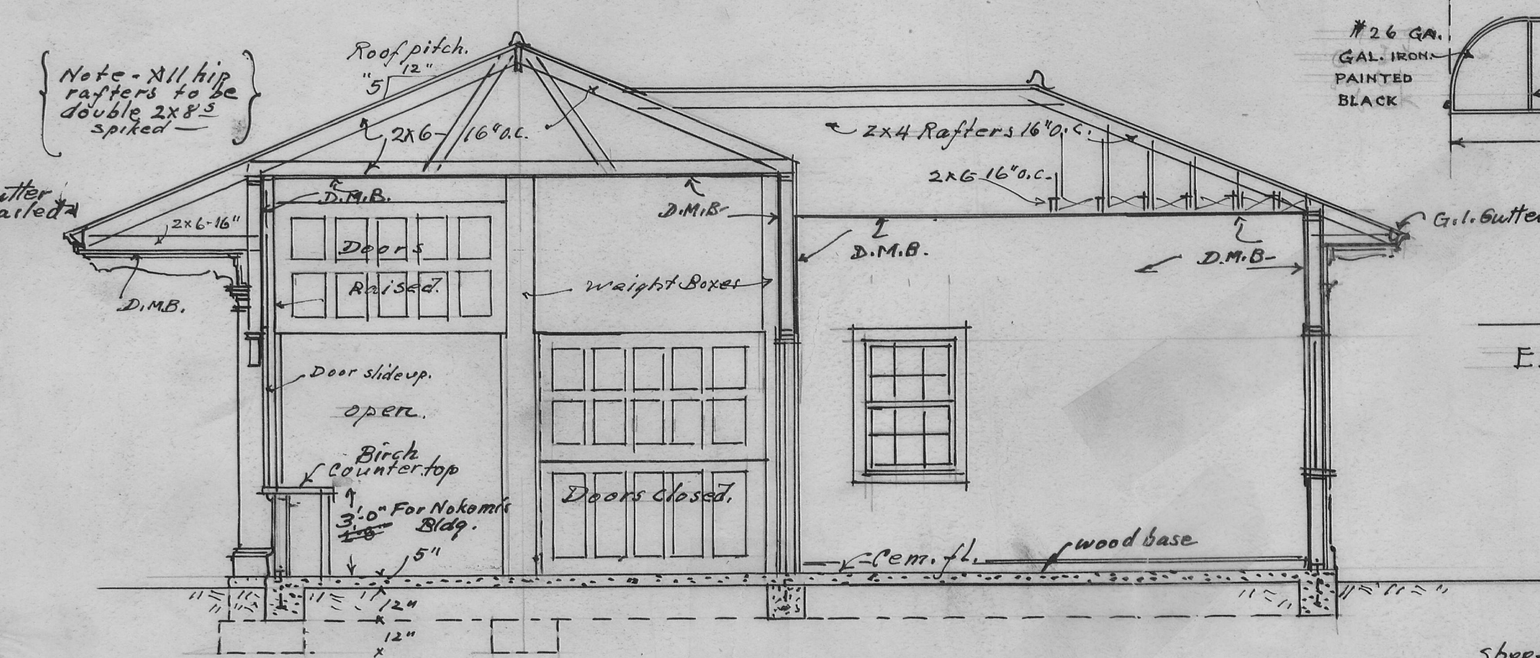
CROSS SECTION
