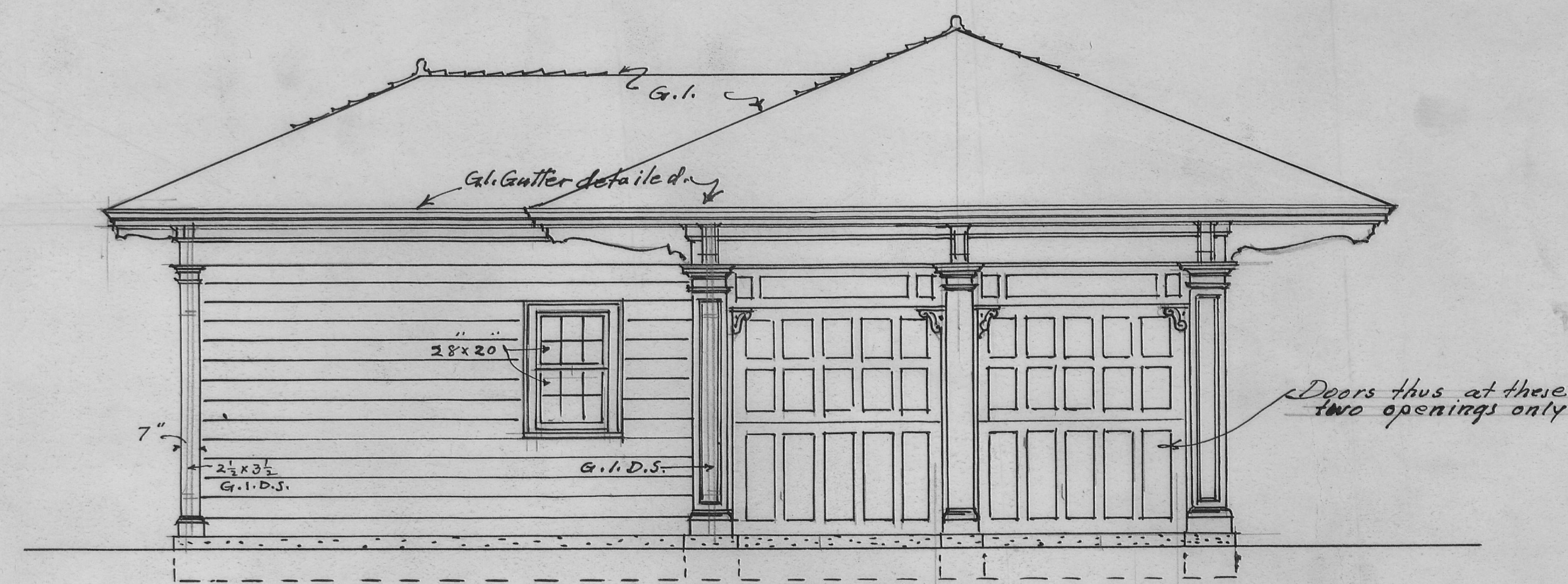
EAST ELEVATION.
